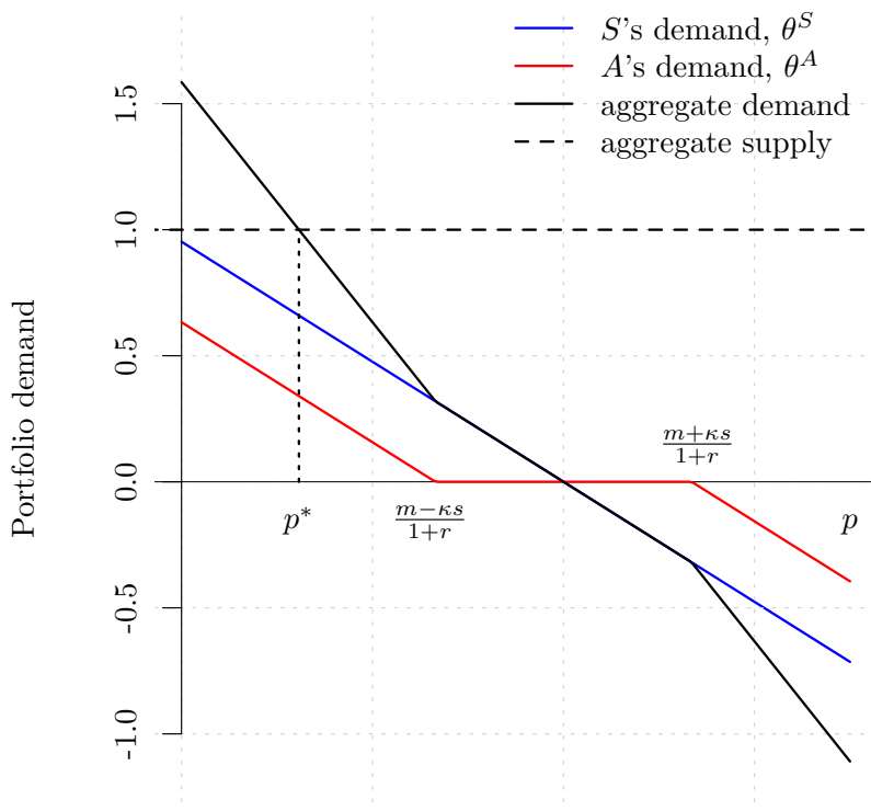
Figure 1: Risky asset demand. The figure shows the risky asset demand \theta^S and \theta^A from equations (8)–(9) as a function of the risky asset price p . The red line denotes type- A 's demand; the blue line type- S 's demand; the black line is aggregate demand; and the dashed line is the aggregate supply of the risky asset. Parameter values: n = 20 , \gamma = 1 , \kappa = 0.15 , \sigma = 0.1 .
